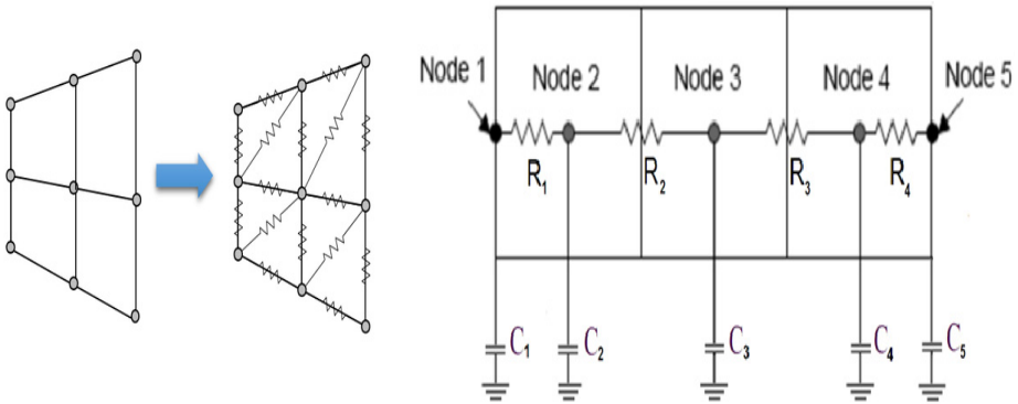
Fig. 9. Thermal RC-network based on the equivalent electrical circuit: Node — network nodes, R — resistances equivalent to thermal radiation, C — capacity equivalent to thermal conductivity between network nodes.
