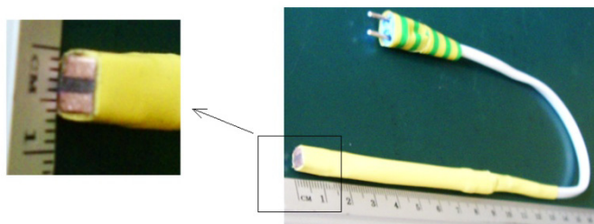
Fig. 3. A bipolar electrosurgical instrument with a split electrode
